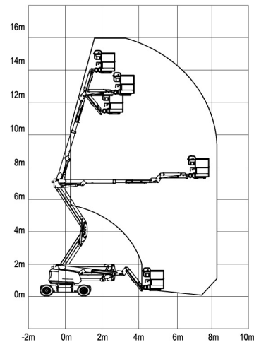
Working Range
